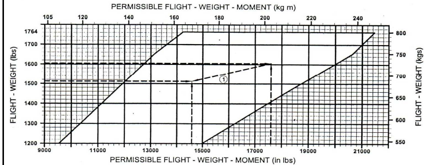
Figure 6.7: Permissible Center of Gravity Range and permissible Flight-Weight-Moment
